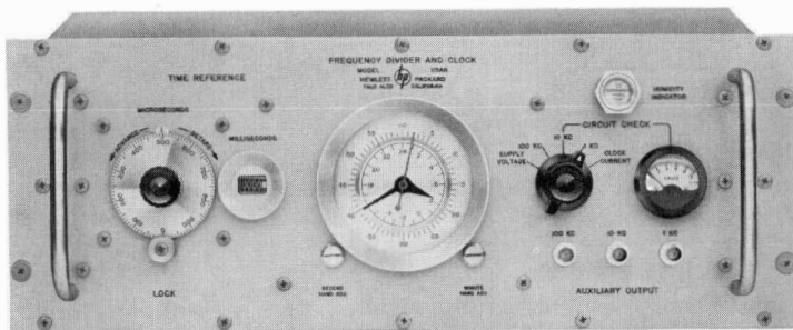
Fig. 1. New -hp- Model 113AR Frequency Divider and Clock simplifies intercomparison of local frequency standards with national standards via broadcast time signals and increases resolution with which such comparisons can be made. Use of instrument with suitable local frequency standard also permits time to be kept on a local basis to within a millisecond. Instrument is fully transistorized and designed with fail-safe provisions.
