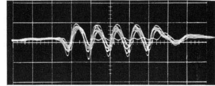
Fig. 6. Multi-exposure oscillogram of received ticks from WWV on 1 millisecond/cm time base. Since ionospheric effects introduce a variable transmission delay into the received signal (in this case of about \frac{1}{2} millisecond), such oscillograms are valuable in establishing arrival-time of earliest-received tick to high resolution.
